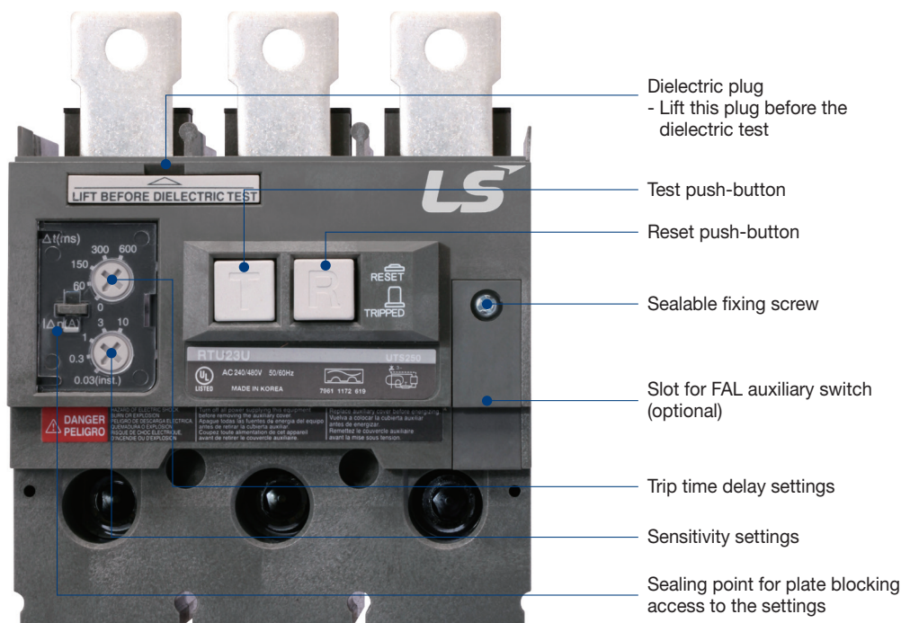
RTU23U, L Circuit breaker combination
