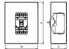
Enclosure Dimensions
